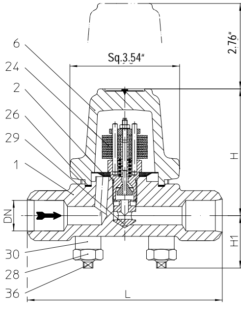
Fig. 600....4 butt welded ends
