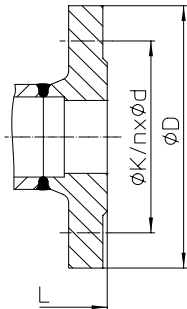
Fig. 600/601....1 flanged
