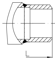
Fig. 600...4 butt welded ends
