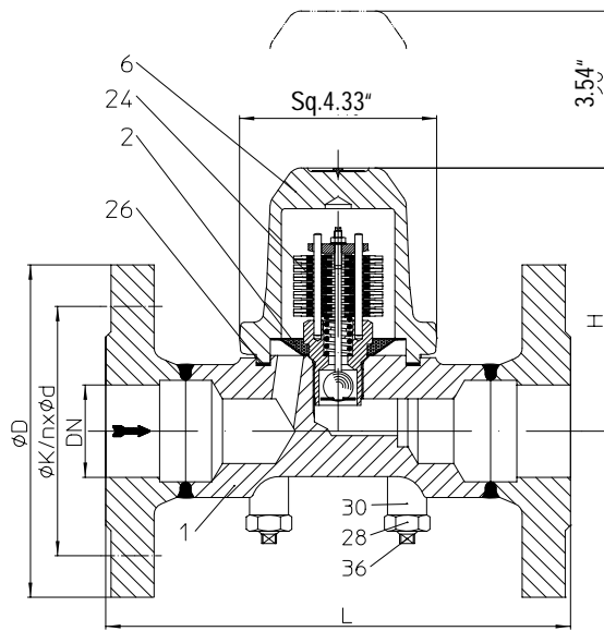
Fig. 600...1 with flanges
